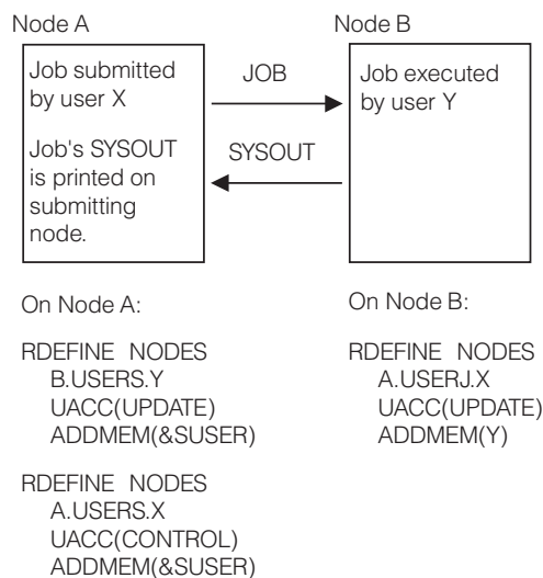
Figure 42: Example: Simple NJE user translation using &SUSER
