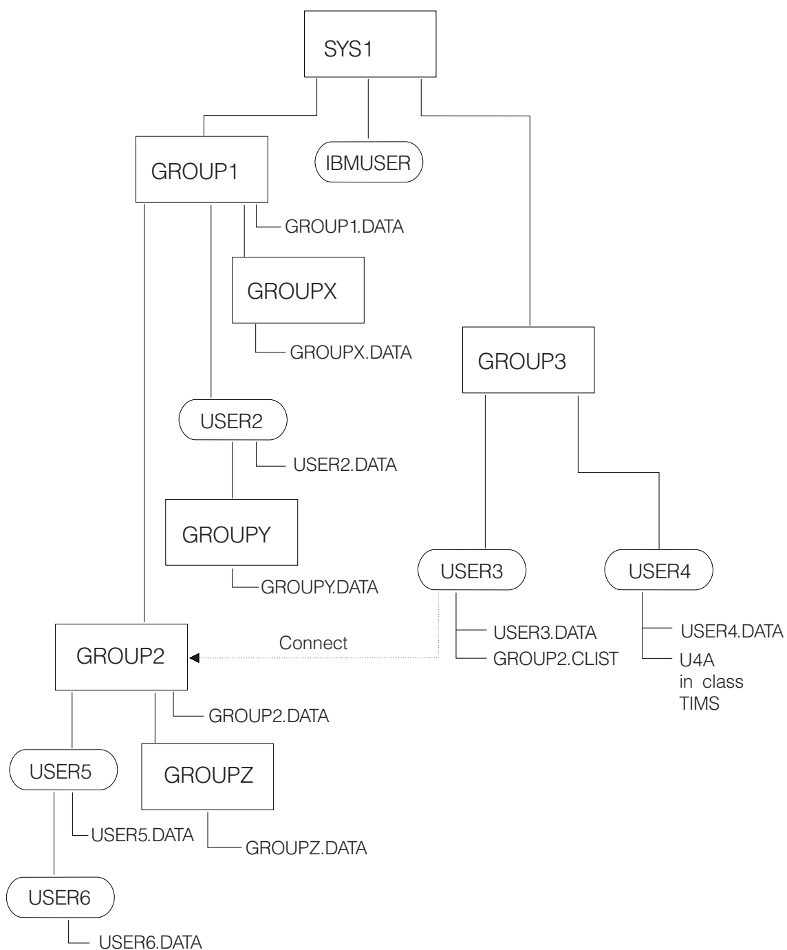
Figure 5: Group-level authority structure
