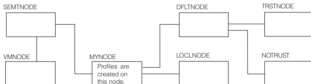
Figure 43: Example: Trusted, semitrusted, and untrusted nodes
